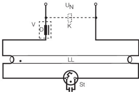
SINGLE CIRCUIT
